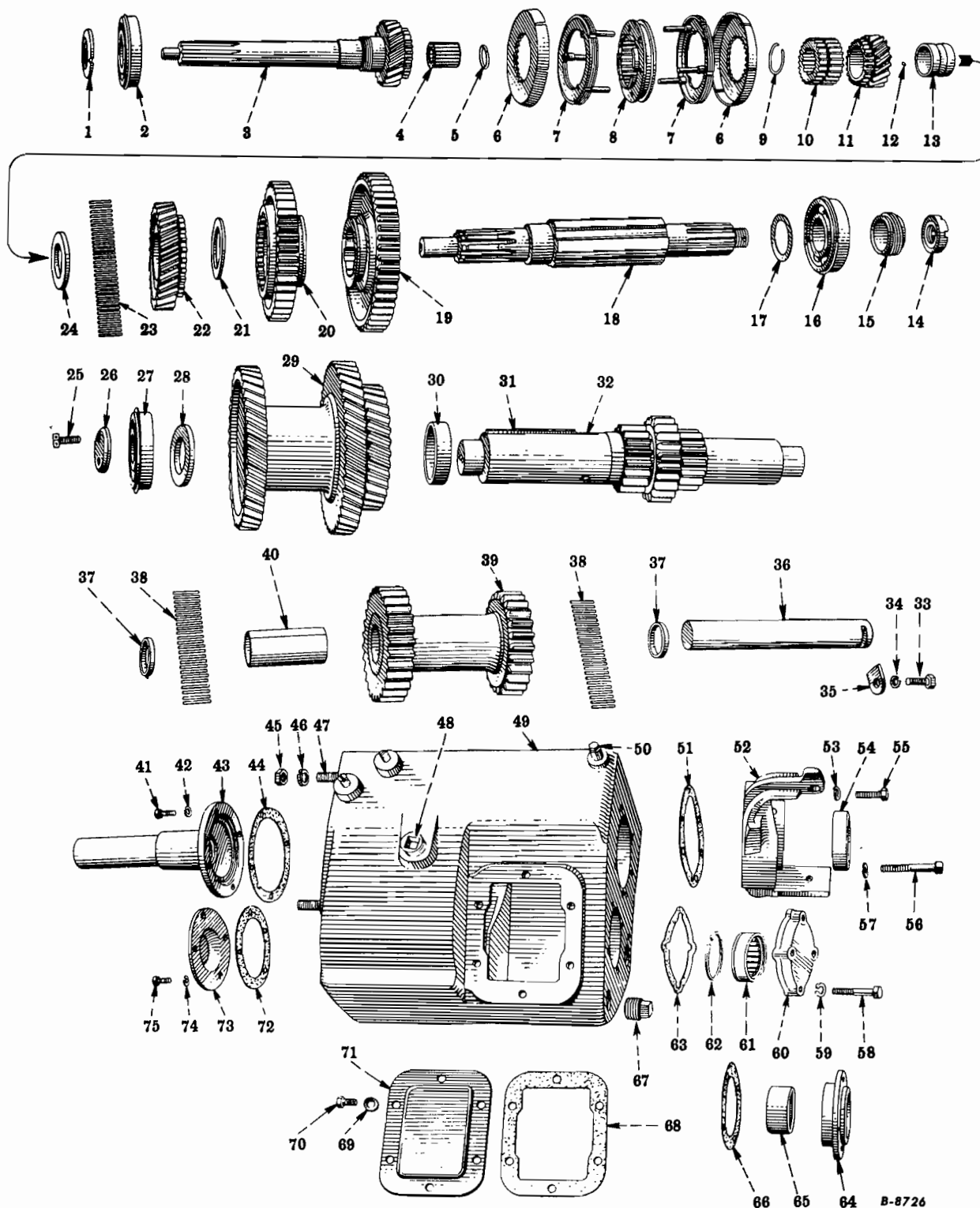
FIG. 13-26 — TRANSMISSION ASSEMBLY (New Process) (5 Speed, Overdrive, Code 1322 And Direct-In-Fifth, Code 1323) (R-160 Series - w/Code 1322 Below 34941) (R-160 Series - w/Code 1323 Below 35684)
