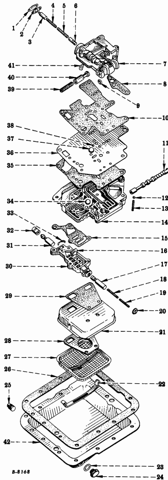
FIG. 13-18 — VALVE BLOCK ASSEMBLY (Automatic Transmission, Code 1374) (R-100, R-110, R-120, R-130 Series) (Below Transmission Serial No. 4750)
