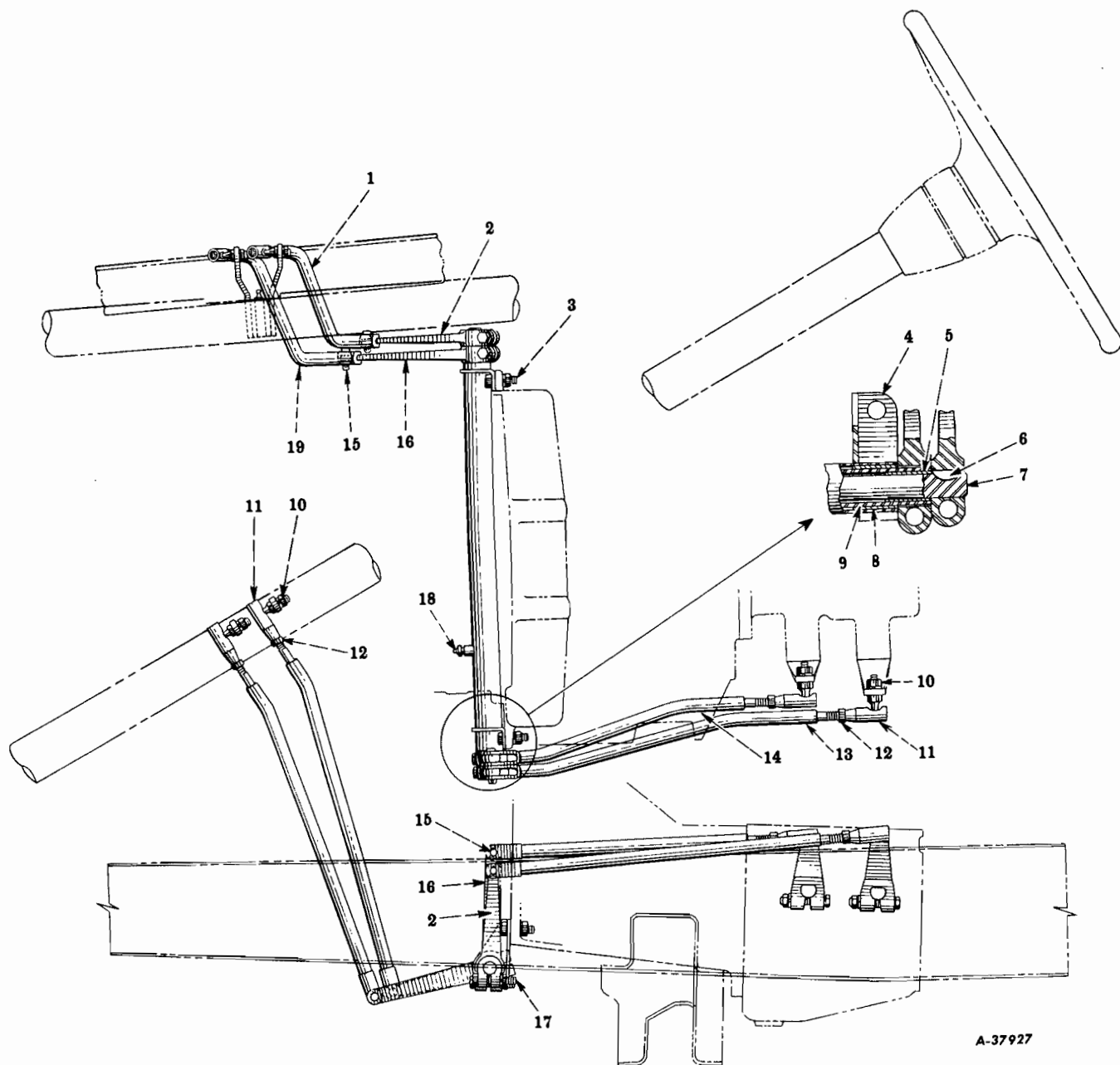
FIG. 13-12 - TRANSMISSION REMOTE CONTROL RODS (Right Hand Drive) (R-110 Series - 47105 Up) (R-120 Series - 9597 Up) (R-100 Series) (Model HNS Transmission, Without Overdrive, Code 1348) (R-100 Series) (R-110 Series - 47105 Up) (With Model HNS Transmission, And With Overdrive, Code 1383)
