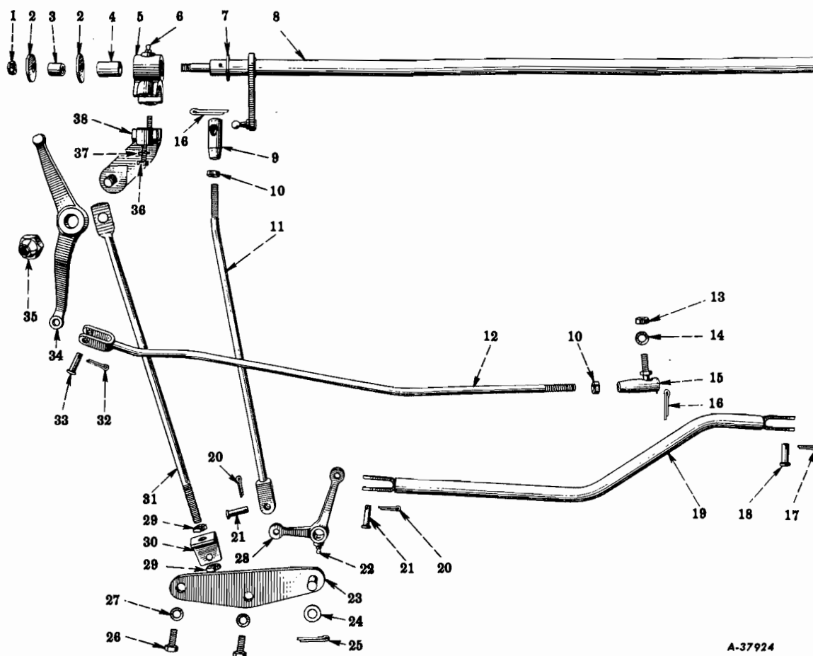
FIG. 13-8 — TRANSMISSION REMOTE CONTROL RODS (Left Hand Drive) (Model T-87 D Transmission, Code 1302) (R-110, R-120, R-130 Series)
