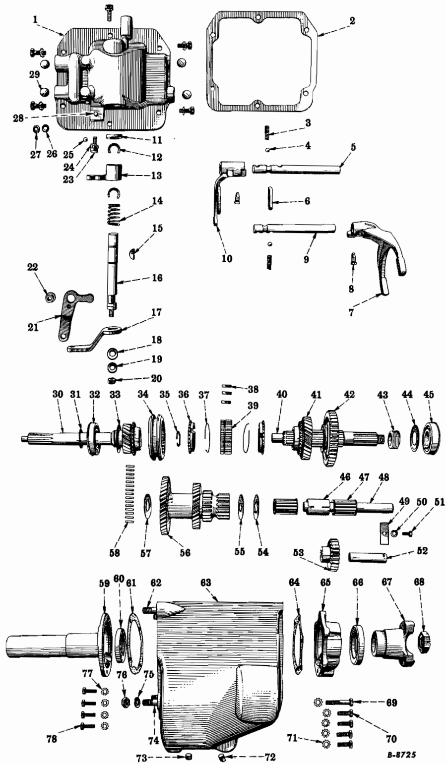
FIG. 13-4 — TRANSMISSION ASSEMBLY (3 Speed, IH Model T-87D, Code 1302) (R-110, R-120, R-130 Series)
