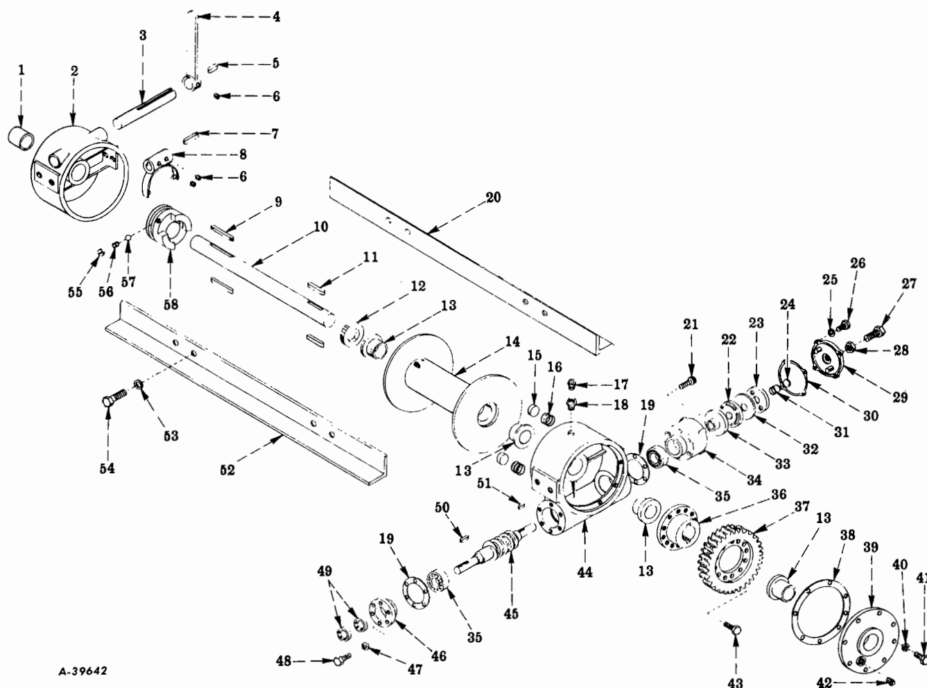
FIG. 13-34A — WINCH (Ramsey Model 700, Code 5375)
