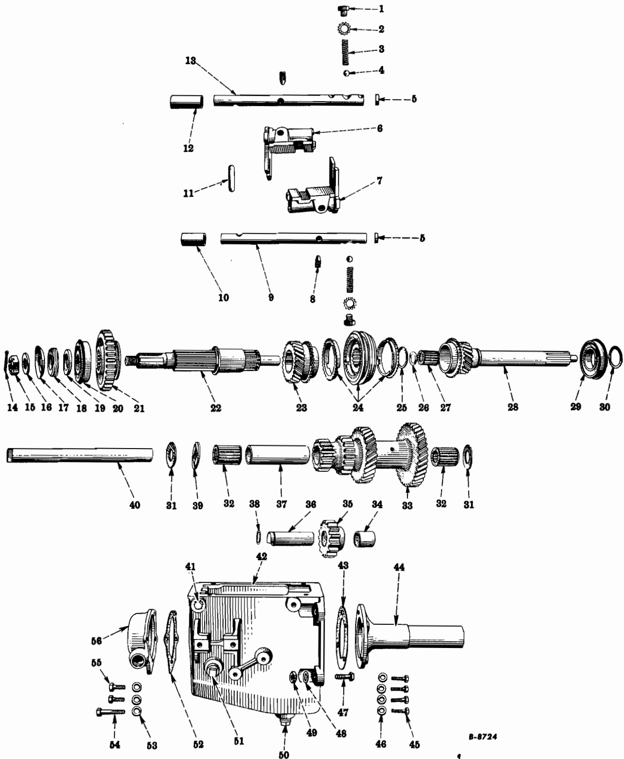
FIG. 13-1 — TRANSMISSION CASE, GEARS AND SHIFT BARS (3 Speed, IH Model HBS, Code 1301) (R-110 Series - Below 47105) (R-120 Series - Below 9597)
