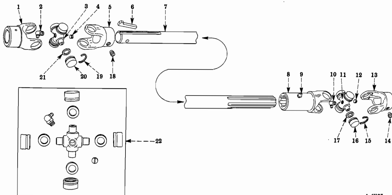
FIG. 13-35 — WINCH DRIVE SHAFT (For Winch Codes 6602, 6604) (R-140-4x4, R-160-4x4)
