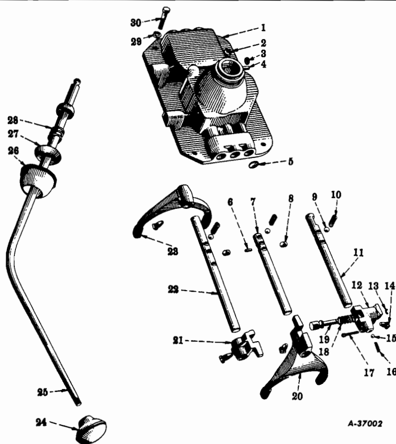
FIG. 13-23 — TRANSMISSION SHIFTING MECHANISM (4-Speed, Model T-98, Code 1303) (R-110, R-120, R-130, R-140-4x4, R-150, R-160, R-160-4x4, RC-160 Series)
