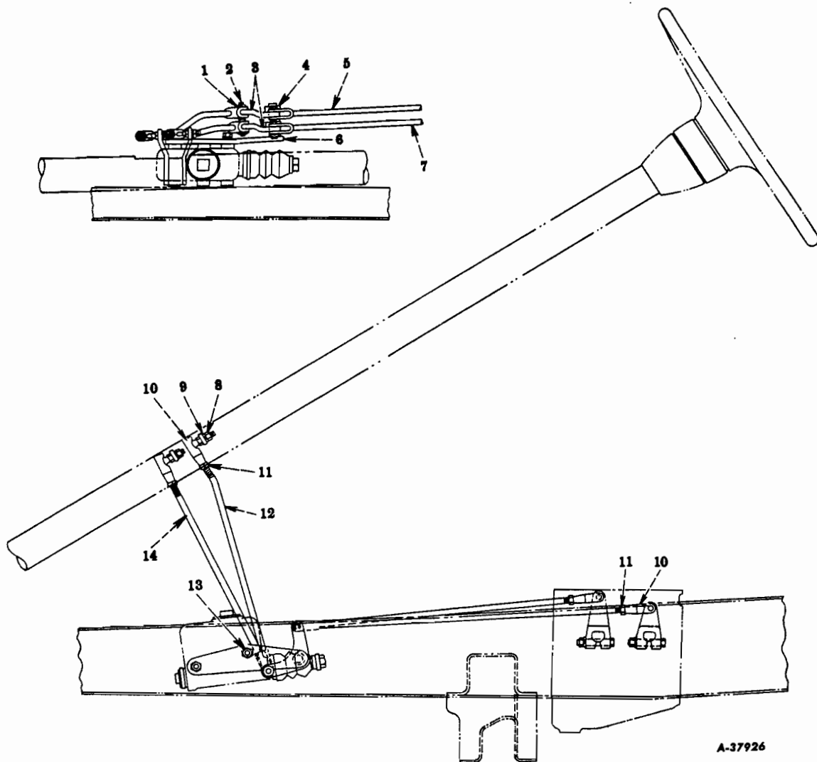
FIG. 13-11 — TRANSMISSION REMOTE CONTROL RODS (Left Hand Drive) (R-110 Series - 47105 Up) (R-120 Series - 9597 Up) (R-100 Series) (Model HNS Transmission, Without Overdrive, Code 1348) (R-100, R-110 Series With HNS Transmission And Overdrive, Code 1383)
