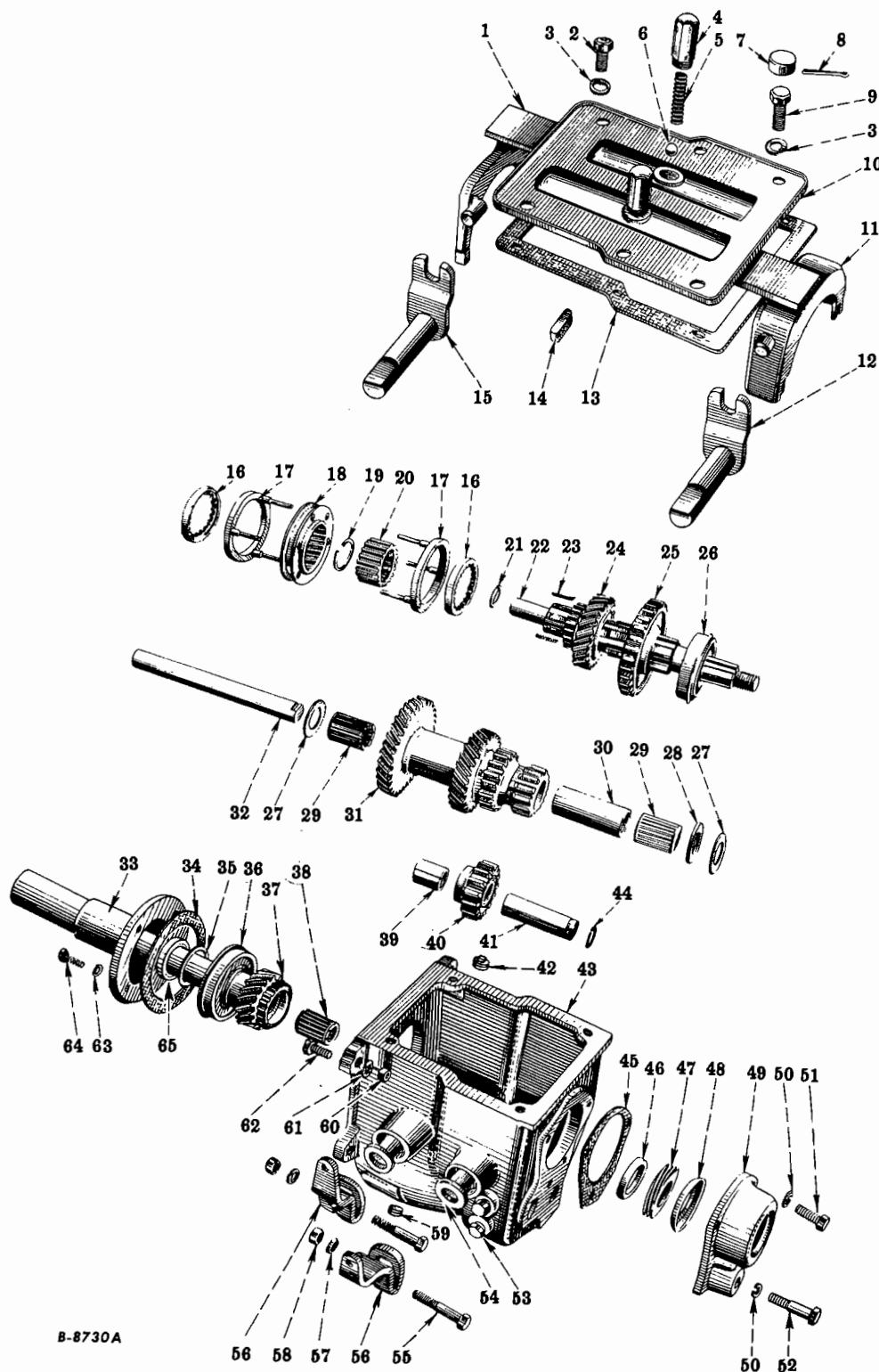
FIG. 13-3 — TRANSMISSION ASSEMBLY (3 Speed, Model HNS, Without Overdrive, Code 1348) (R-100 Series) (R-110 Series - 47105 and Up) (R-120 Series - 9597 and Up)
