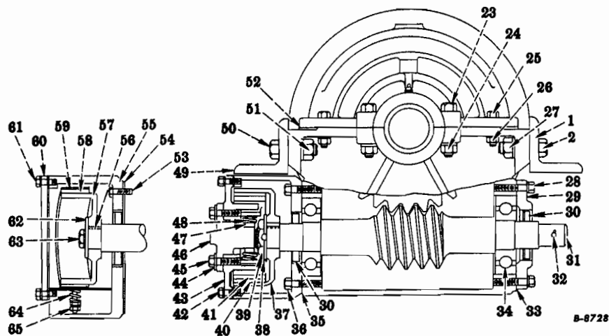
FIG. 13-34 - WINCH, FRONT MOUNTED (R-140-4x4 Series - Model 12-G, Code 6602) (R-160-4x4 Series - Model 18-G, Code 6604)
