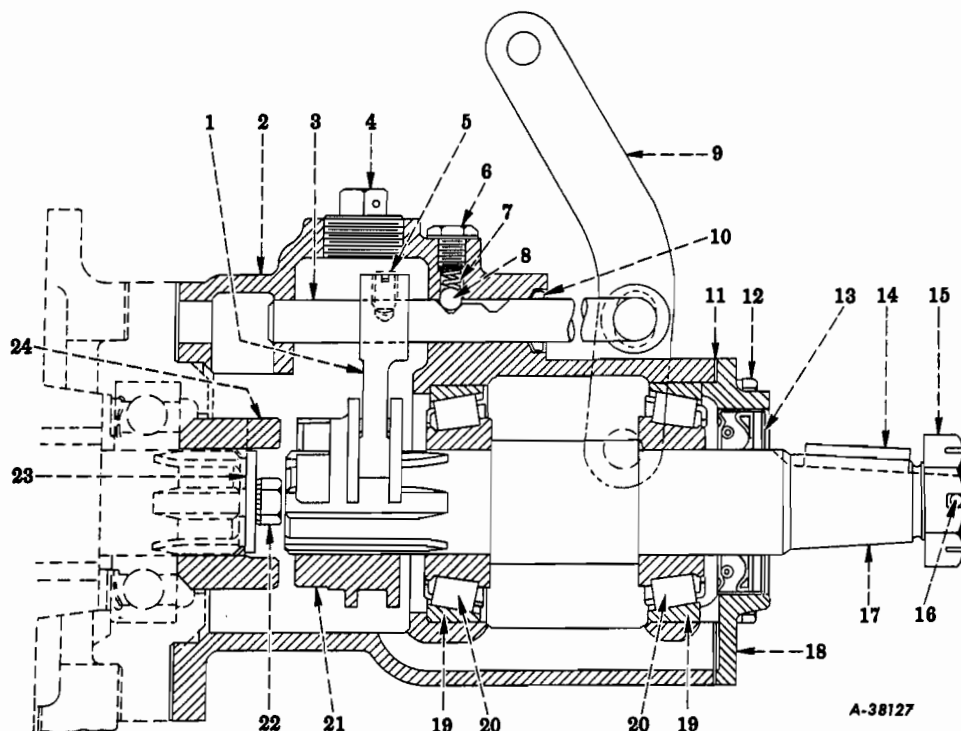
FIG. 13-33 — TRANSFER CASE POWER TAKE-OFF (Code 1392)
