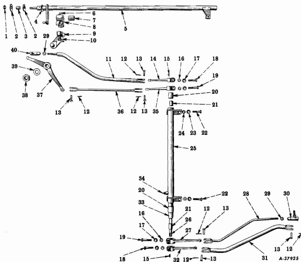
FIG. 13-9 - TRANSMISSION REMOTE CONTROL RODS (Right Hand Drive) (Model T-87D, Code 1302) (R-110, R-120, R-130 Series)
