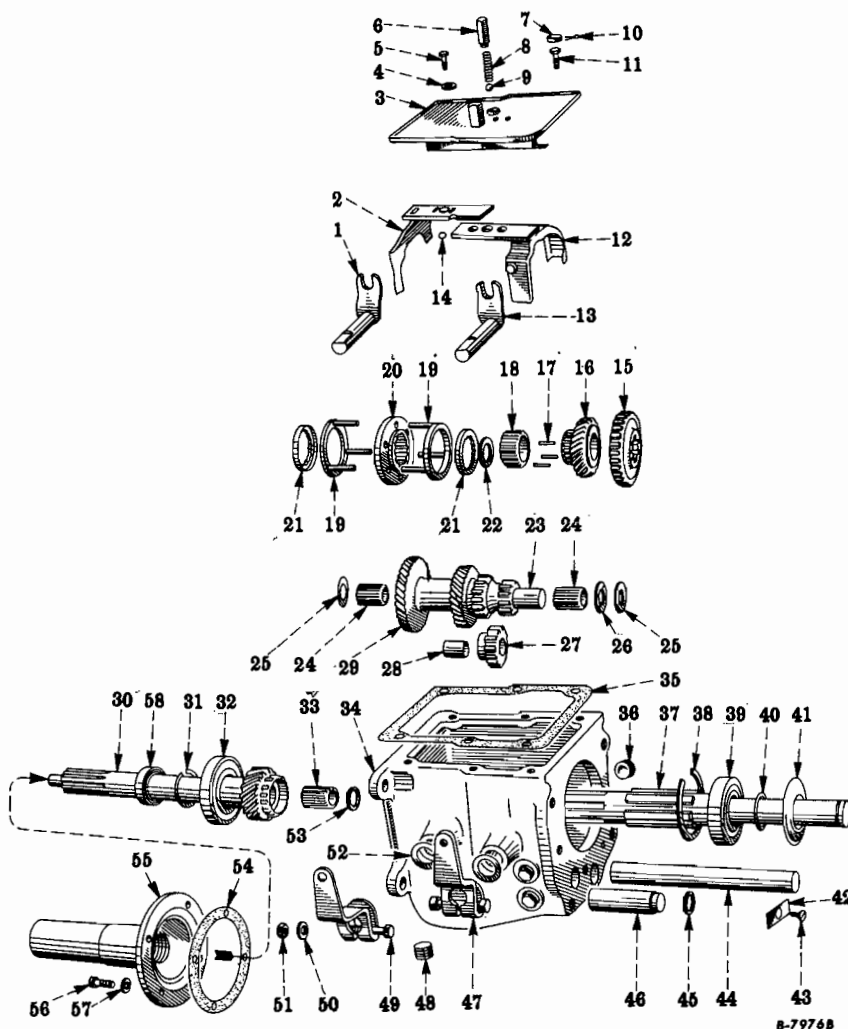
FIG. 13-13 — TRANSMISSION ASSEMBLY (3 Speed, Model HNS, With Overdrive, Code 1383) (R-100, R-110 Series)
