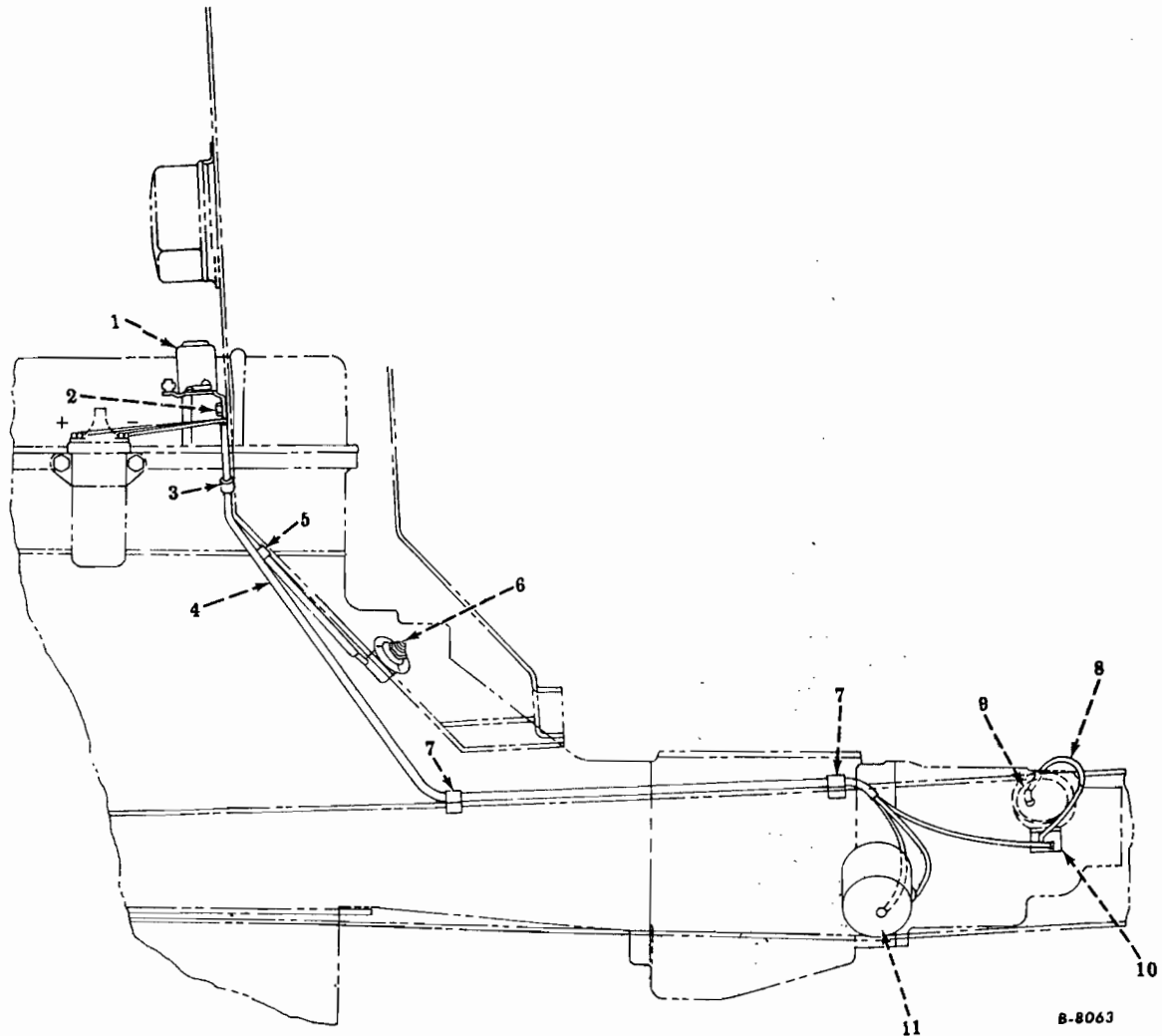
FIG. 13-15 - OVERDRIVE WIRING (For 3 Speed, Model HNS With Overdrive, Code 1383) (R-100, R-110 Series)
