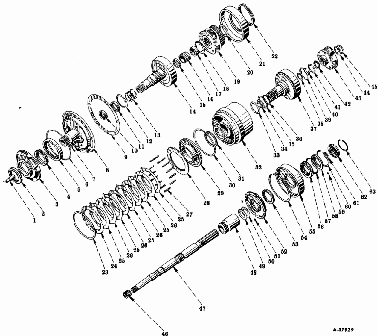
FIG. 13-17 — FRONT PUMP AND COLLECTOR RING, MAINSHAFT, AND MULTIPLE DISC CLUTCH (Automatic Transmission, Code 1374) (R-100, R-110, R-120, R-130 Series)
