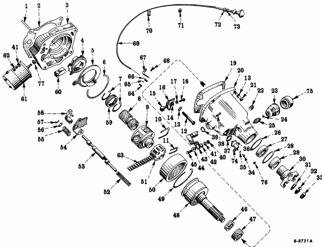
FIG. 13-14 — OVERDRIVE UNIT (3 Speed, Model HNS, With Overdrive, Code 1383) (R-100, R-110 Series)
