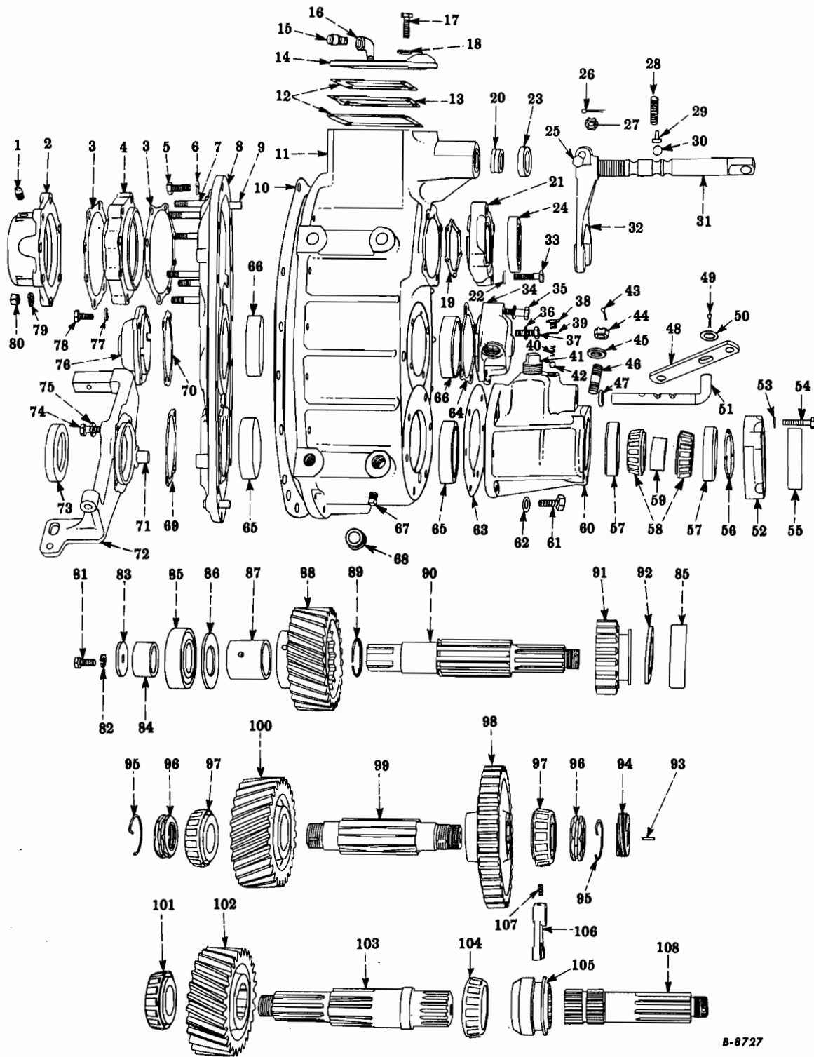
FIG. 13-29 — TRANSFER CASE (Timken, Model T-32) (R-140-4x4, R-160-4x4 Series)
