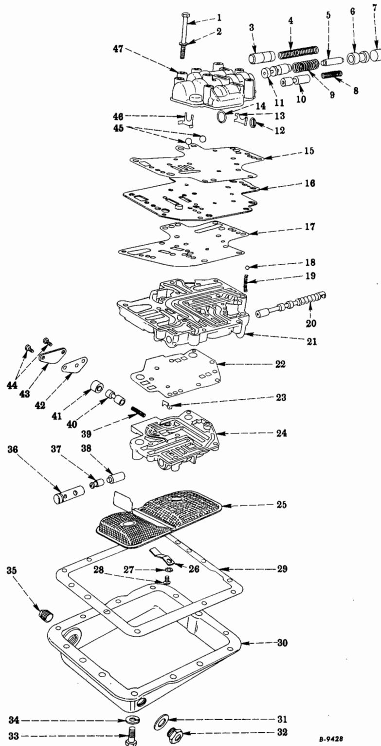
FIG. 13-18A — TRANSMISSION VALVE BLOCK ASSEMBLY (Automatic Transmission, Code 1374) (Transmission Serial No. 4750 Up) (R-100, R-110, R-120, R-130 Series)
