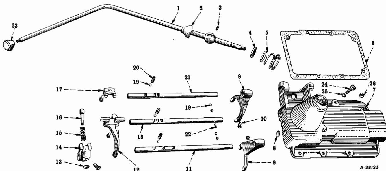
FIG. 13-27 — TRANSMISSION CONTROL HOUSING (New Process) (5 Speed, Overdrive, Code 1322 And Direct-In-Fifth, Code 1323) (R-160 Series w/Code 1322 Below 34941) (R-160 Series w/Code 1323 Below 35684)
