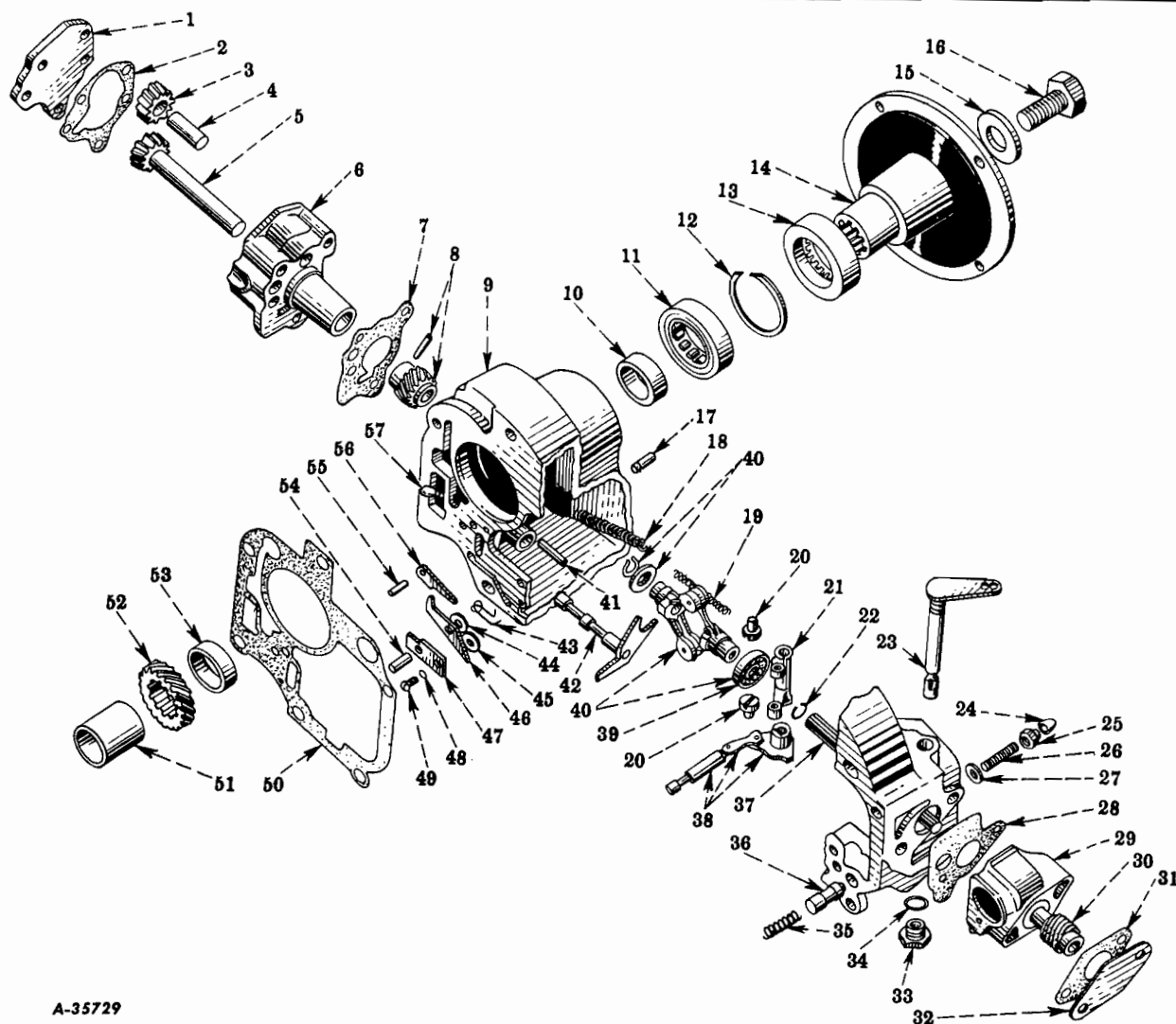
FIG. 13-19 — EXTENSION CASE, GOVERNOR, REAR OIL PUMP AND SPEEDOMETER GEAR HOUSING (Automatic Transmission, Code 1374) (R-110, R-100, R-120, R-130 Series)
