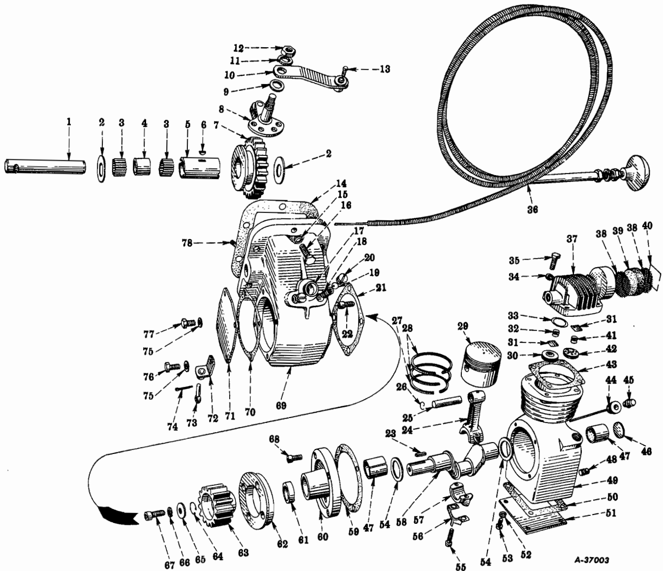
FIG. 13-28 - TIRE PUMP (Code 1361) (R-160 Series)
