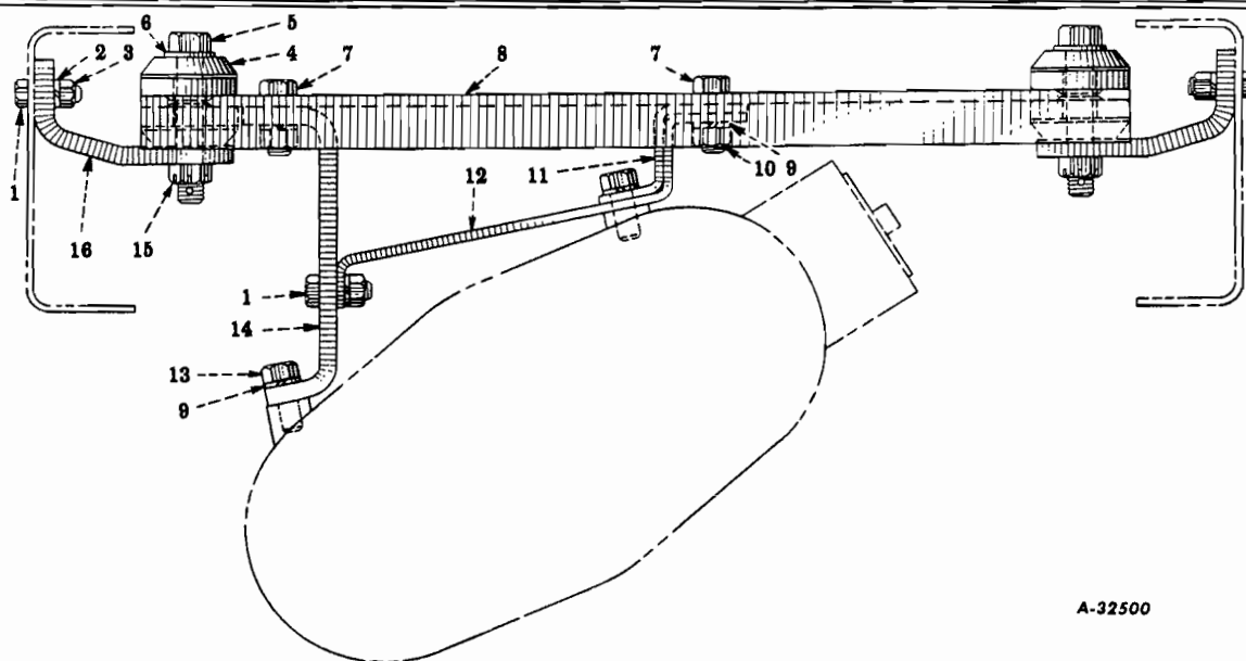
FIG. 13-30 — TRANSFER CASE MOUNTING (R-140-4x4, R-160-4x4 Series)
