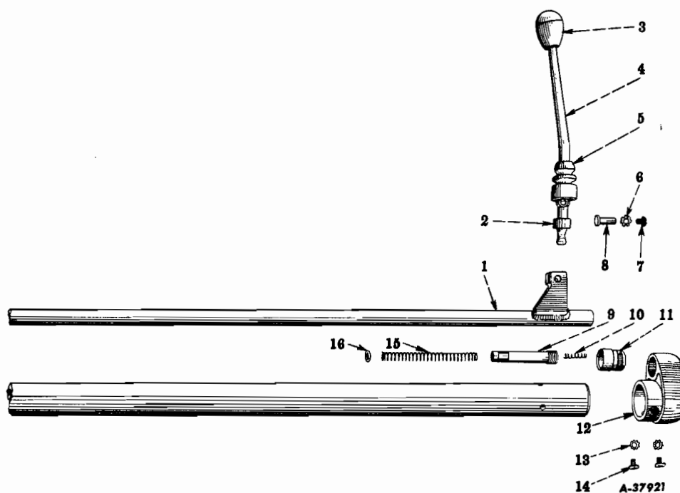
FIG. 13-5 — TRANSMISSION REMOTE CONTROL
