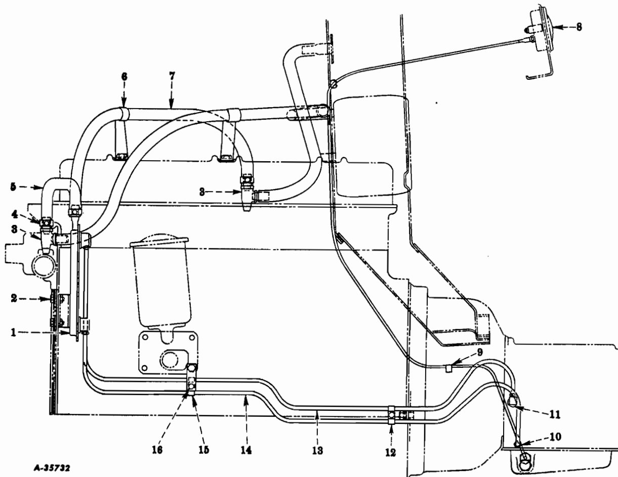
FIG. 13-20 — TRANSMISSION OIL COOLER (Code 1384) AND OIL TEMPERATURE GAUGE (Code 1385) (For Automatic Transmission, Code 1374) (R-100, R-110, R-120, R-130 Series)
