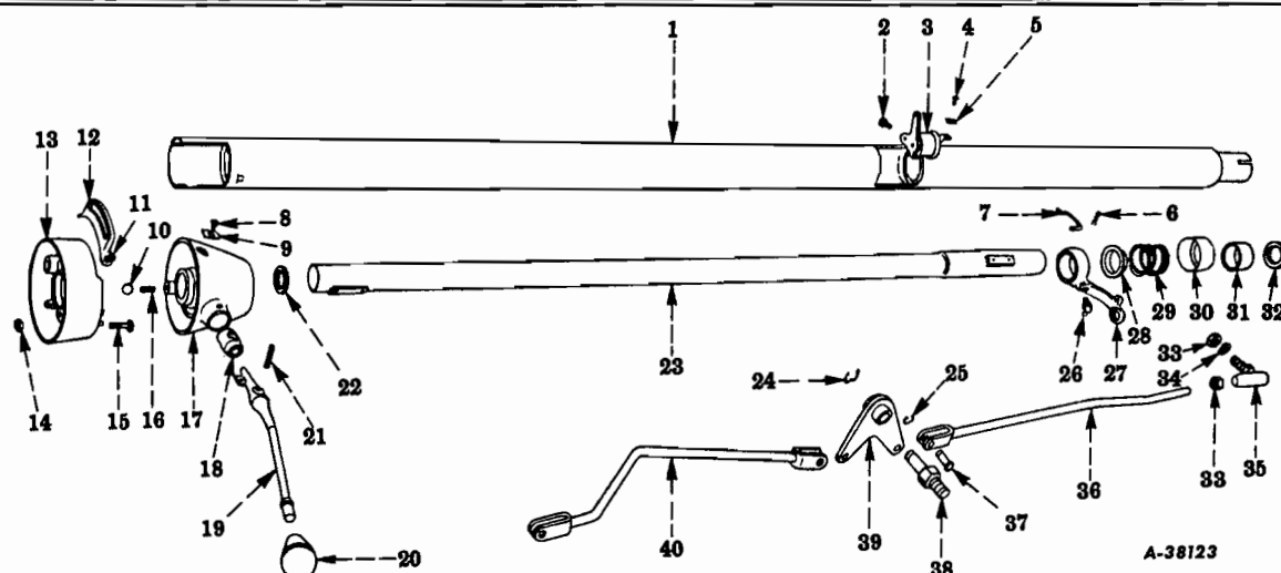
FIG. 13-21 - TRANSMISSION REMOTE CONTROL AND RODS (Automatic Transmission, Code 1374) (R-100, R-110, R-120, R-130 Series)
