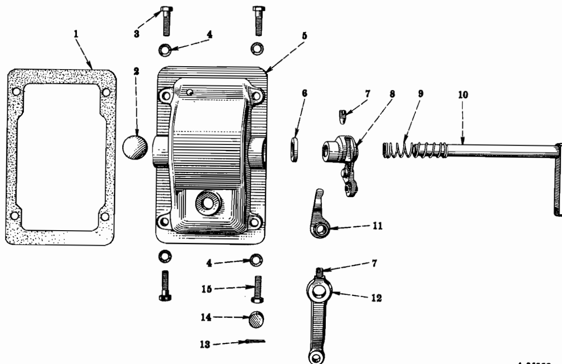
FIG. 13-2 — TRANSMISSION CONTROL HOUSING (3 Speed, IH Model HBS, Code 1301) R-110 Series - Below Chassis No. 47105 R-120 Series - Below Chassis No. 9597
