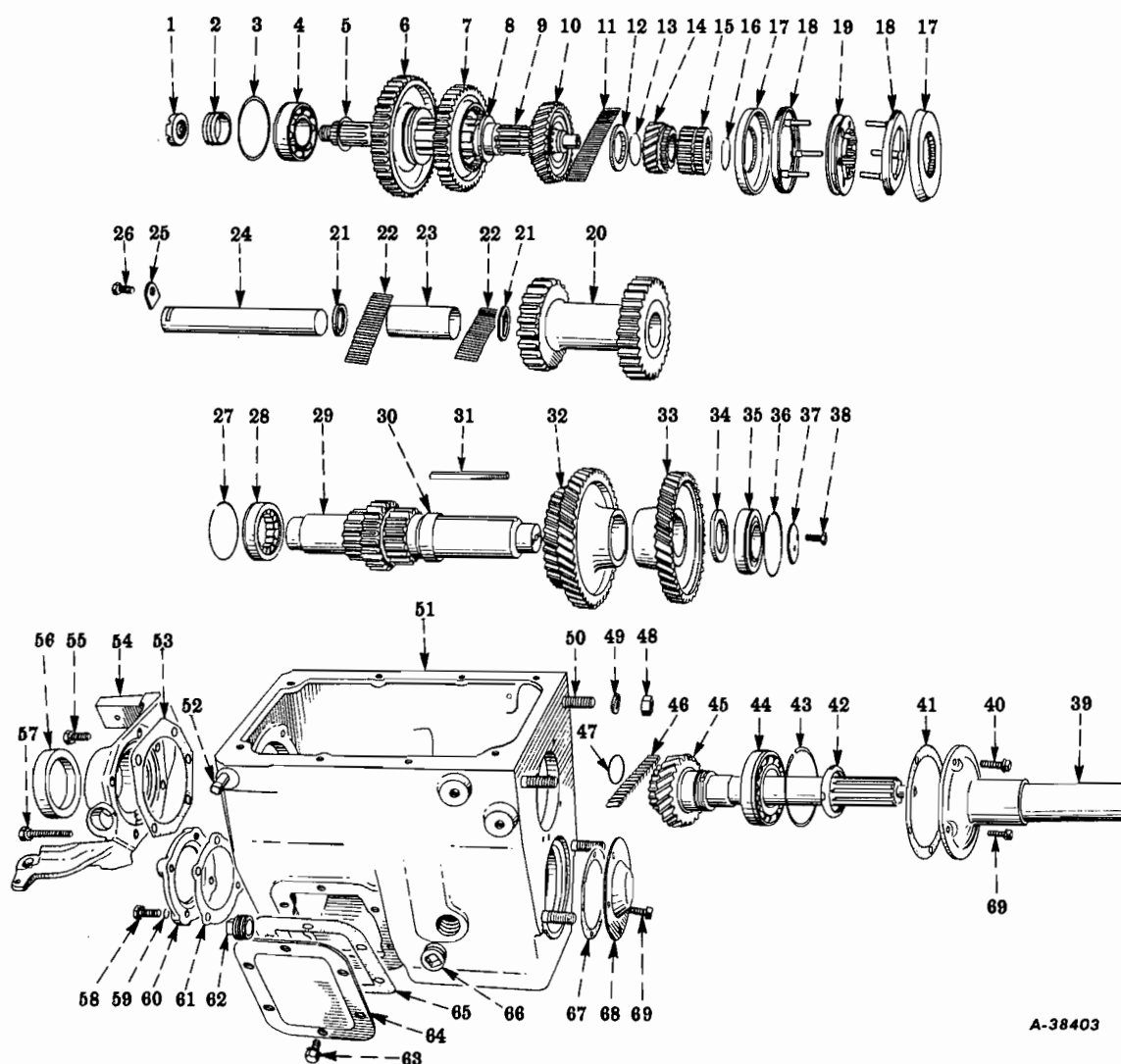
FIG. 13-26A — TRANSMISSION CASE AND GEAR (New Process) (5-Speed Overdrive, Code 1305; Direct-In-Fifth, Code 1306) (R-160 Series - w/Code 1305, 34941 Up And w/Code 1306, 35684 Up) (RC-160 Series - 501 Up)
