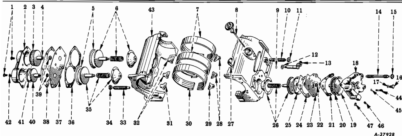
FIG. 13-16 — TRANSMISSION CASE, SERVOS, BRAKE BANDS AND SELECTOR LEVER (Automatic Transmission, Code 1374) (R-100, R-110, R-120, R-130 Series)
