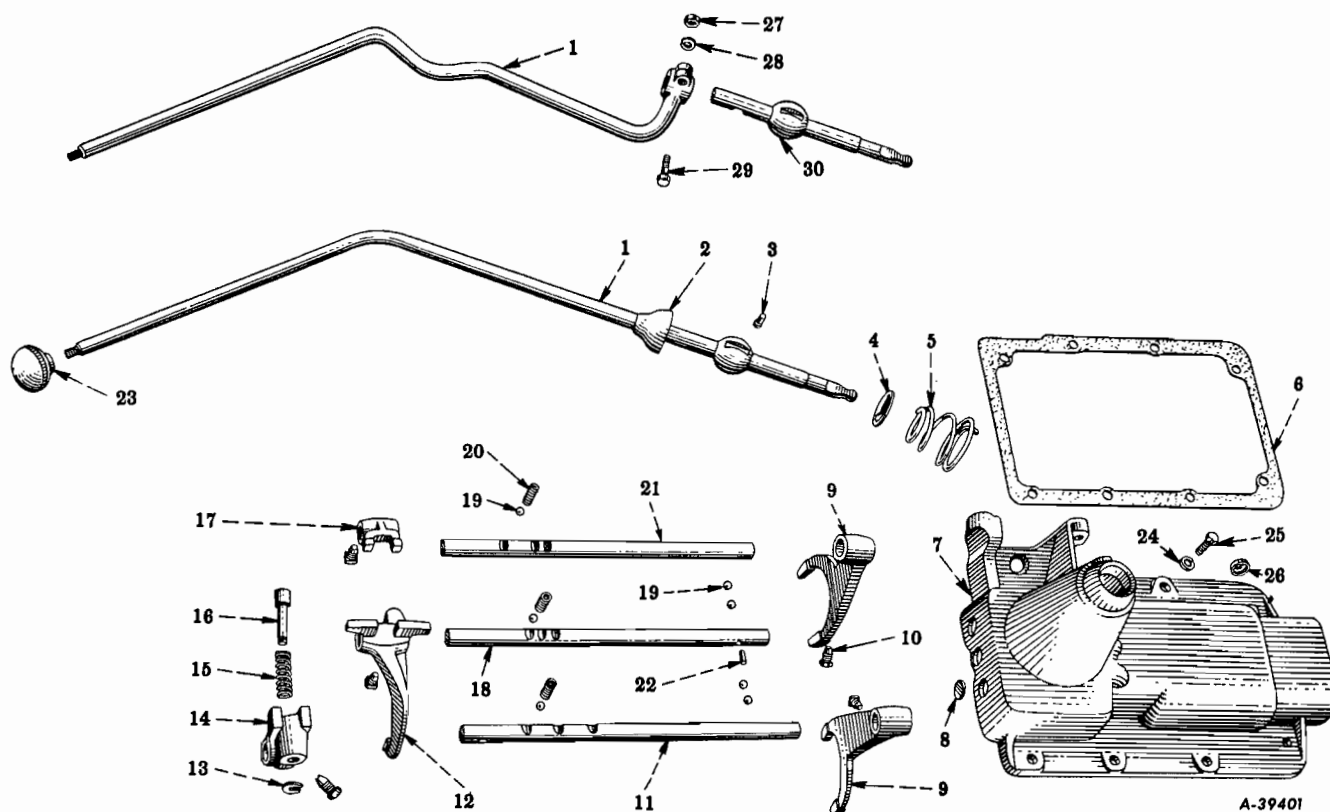
FIG. 13-27A — TRANSMISSION SHIFTING MECHANISM (New Process)
