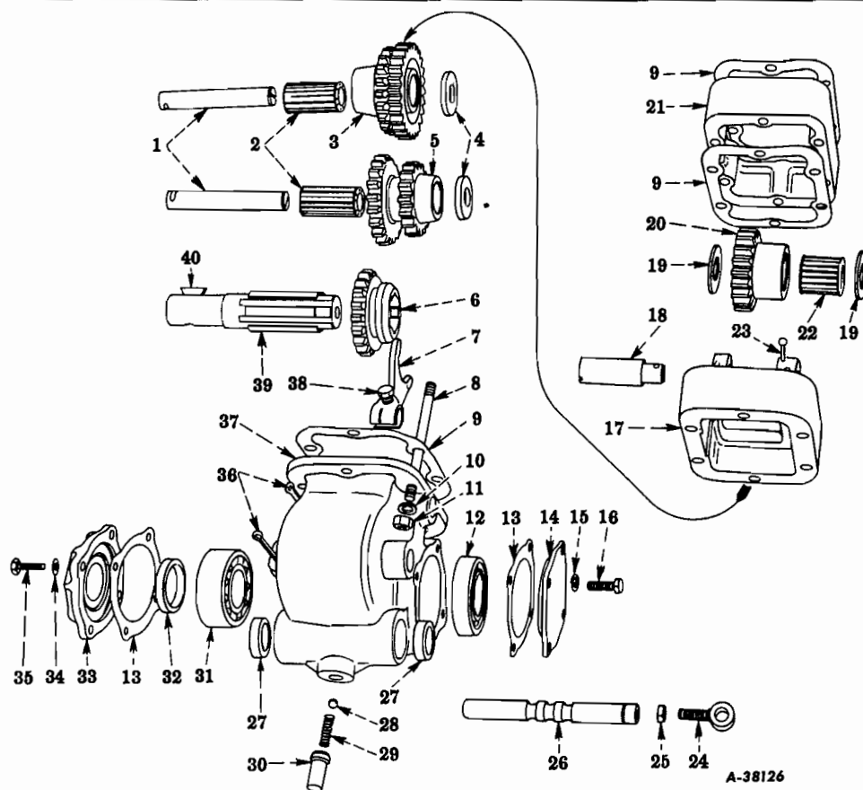
FIG. 13-31 — TRANSMISSION POWER TAKE-OFF (For Winch, Codes 5376, 6602, 6604)
