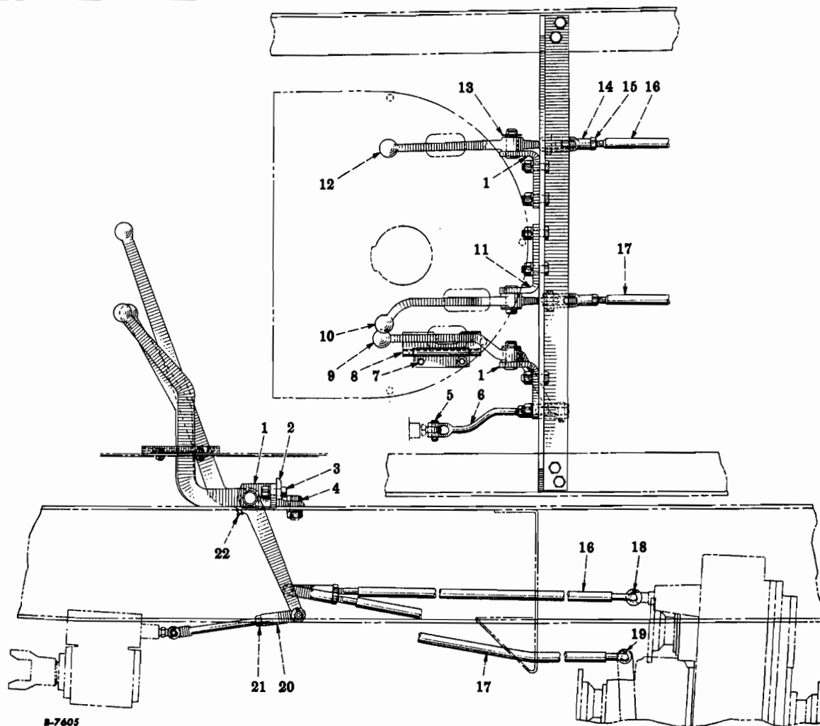
FIG. 13-32 — TRANSFER CASE AND TRANSMISSION POWER TAKE-OFF CONTROLS (R-140-4x4, R-160-4x4 Series)
