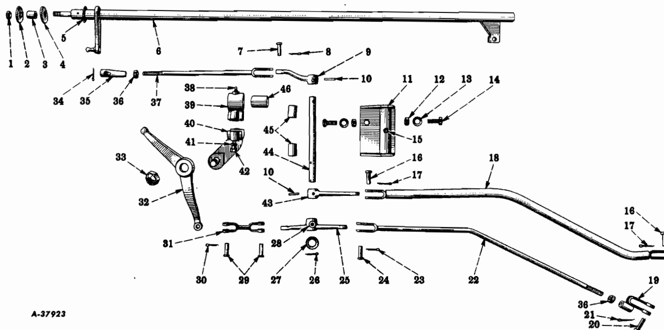
FIG. 13-7 - TRANSMISSION REMOTE CONTROL RODS (Right Hand Drive) (Model HBS Transmission, Code 1301) (R-110 Series - Below 47105) (R-120 Series - Below 9597)
