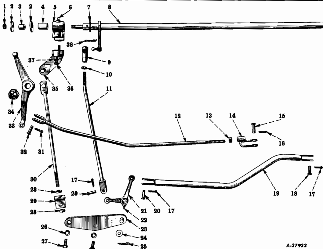
FIG. 13-6 - TRANSMISSION REMOTE CONTROL RODS (Left Hand Drive) (Model HBS Transmission, Code 1301) (R-110 - Below 47105) (R-120 - Below 9597)
